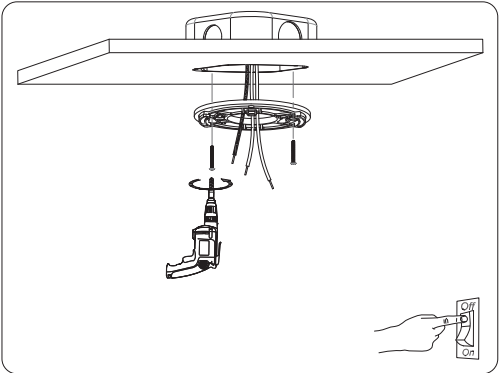
1. Cut off the main power supply. Then secure the mounting bracket to the J-box by using the screws in the accessory pack.
