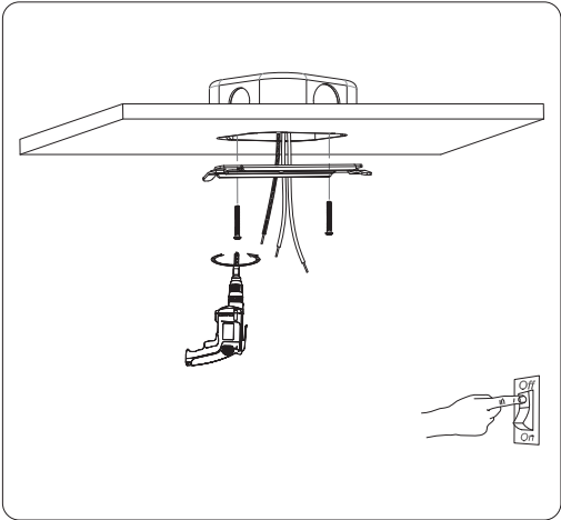
1. Cut off the main power supply. Then secure the mounting bracket to the J-box by using the screws in the accessory pack.
