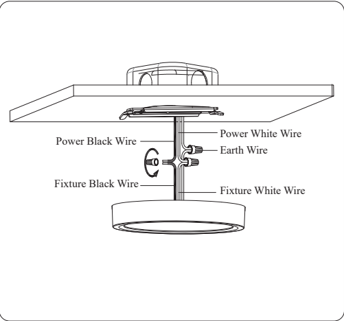
2. Use the wire nut provided in the accessory kit to connect the power cord of the fixture and the J-box.
