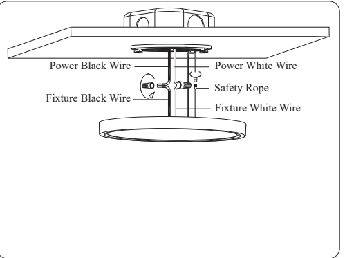
2. Use the wire nut provided in the accessory kit to connect the power cord of the lamp and the J-box. (Remark: 12"/ 16" lamp has a safety rope. Please pass the safety rope though the mounting bracket, then tighten the connecting terminal.)
