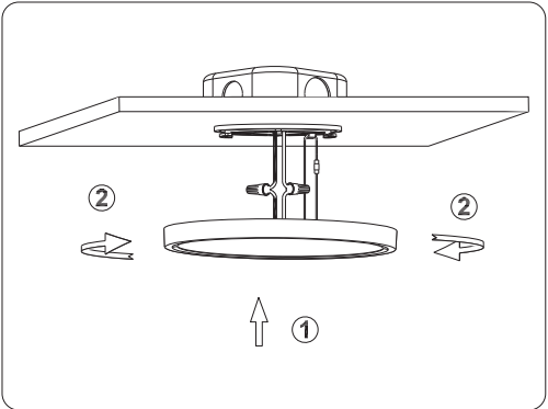
3. Carefully place all the wires into the J-box. Align the fixture's locking slots with the mounting bracket clips, then push the fixture upward toward the ceiling in the direction of the arrow and rotate it until it is fully fixed onto the mounting bracket.
