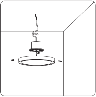
4. Connect the lamp input line and the hanging power line with the rotating terminal, align the lamp slot with the buckle of the mounting bracket and install it upwards, and rotate the lamp to a completely fixed position.
