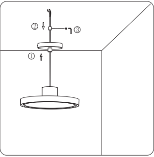
5. Pass the hanging power cable through the center hole of the ceiling plate, adjust the fixing cable clip to an appropriate length and tighten it with the screw.
