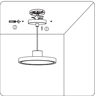
8. Fix the ceiling plate to the hanging bracket with screws.
