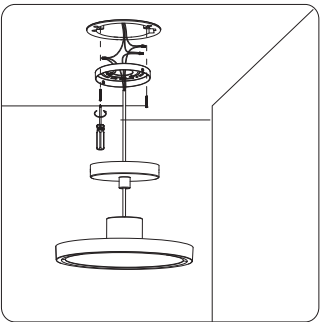
7. Fix the hanging bracket to the junction box with screws.
