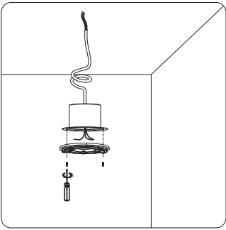
3. Connect the ground wire on the bracket to the ground wire in the hanging accessory with toothpaste cap screw terminal.
