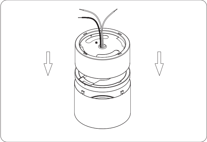
1. Install the lamp and inner liner into the decorative trim in sequence.
