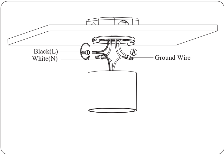
4. Connect the lamp wire and power with wire nuts. If the lamp has a ground wire, connect it to position (A).
