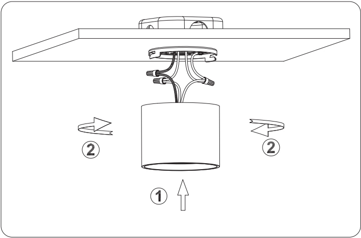
5. Tuck all wires into the junction box. Align the card slot of the lamp’s mounting bracket with the mounting bracket, push the lamp toward the ceiling (1), then rotate it in the direction of the arrow (2) until it is fully fixed to the mounting bracket.
