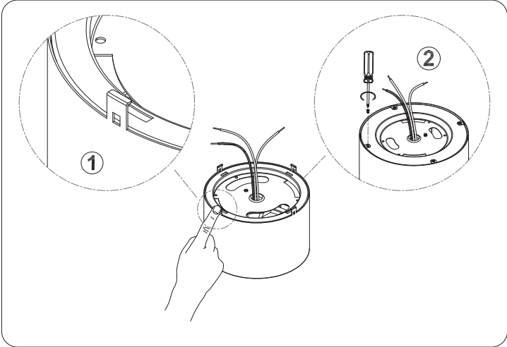
2. Snap on the clips into the lamp's groove. for some models, this position uses a locking screw (as shown in Figure 2).
