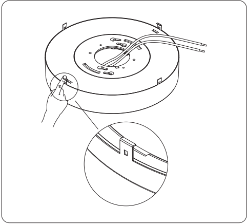
2.Press the hanging ears against the back of the lamp fixture using your fingers or a tool to secure it in place.
