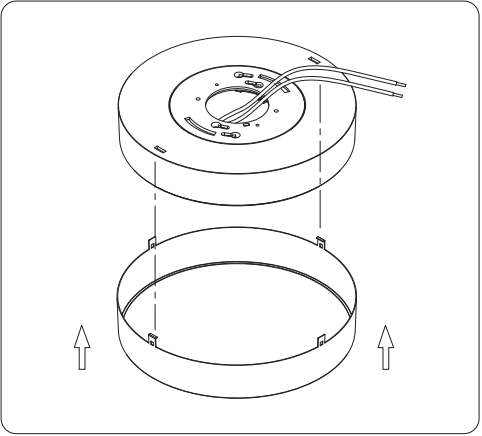
1.Align the hanging ears of the decorative ring with the grooves on both sides of the lamp fixture.
